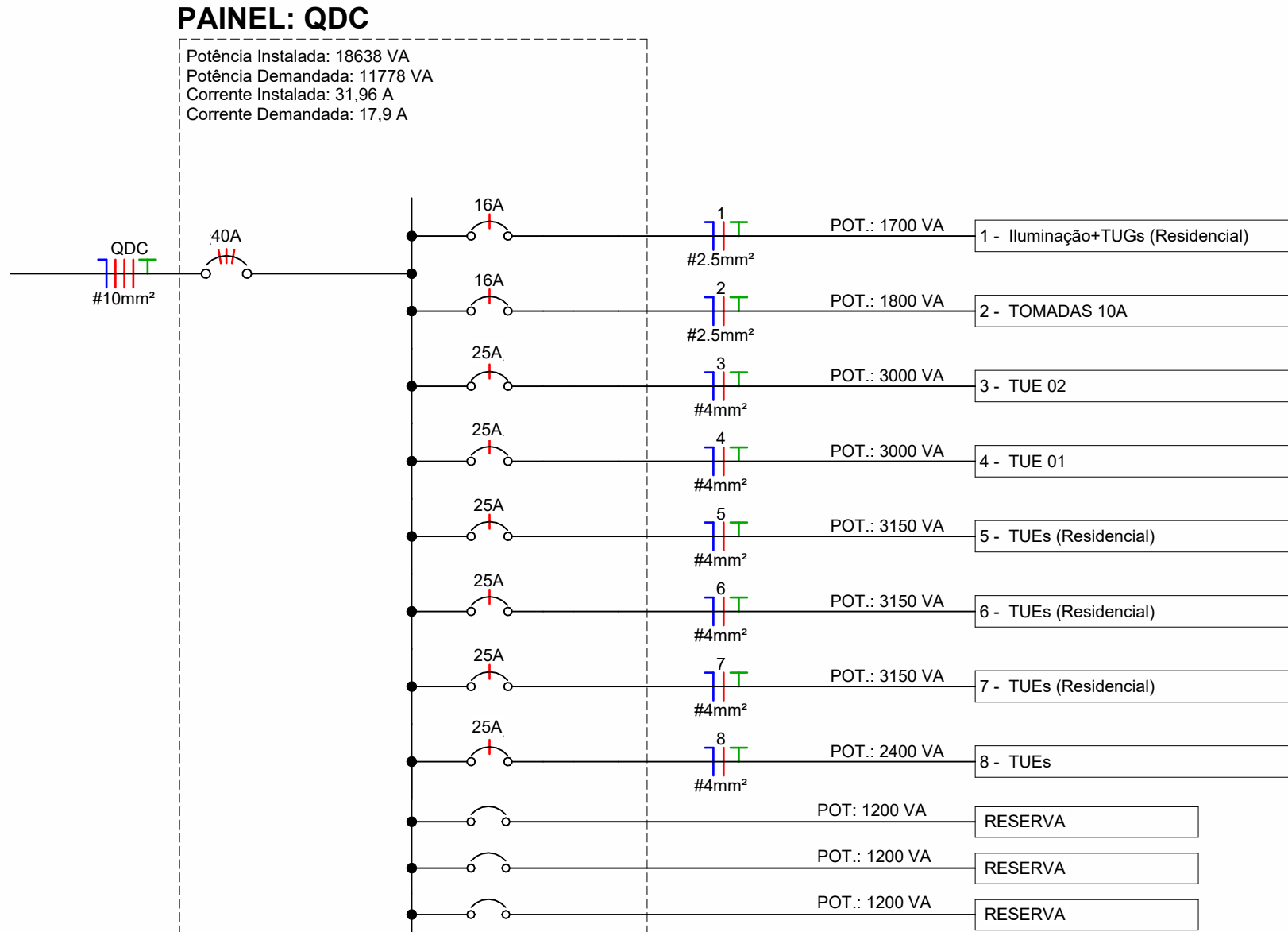
Diagrama Unifilar
